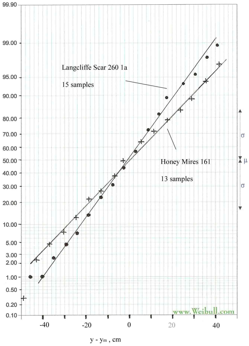
FIGURE 7 Probability plots
