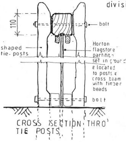
group CROSS SECTION
